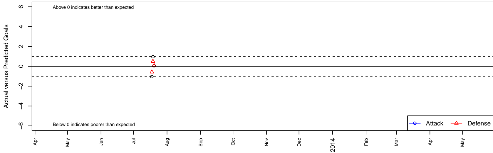
TN FC Alliance B98 Dots are actual minus expected GF (blue circles) and GA (red triangles). Blue line is smoothed change in attack strength. Red is smoothed change in defense strength.
